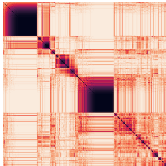
tp15 (PAC=0.37, 2000 genes)
