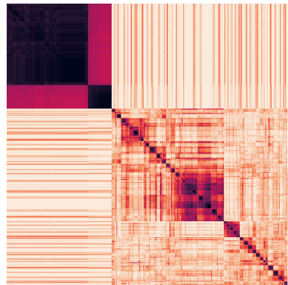
tp11 (PAC=0.39, 2000 genes)
